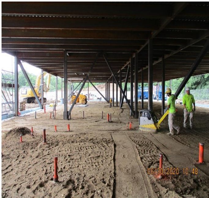
COMPACTION OF BUILDING B SUBGRADE
